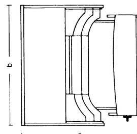
13 Plan of free-standing console
